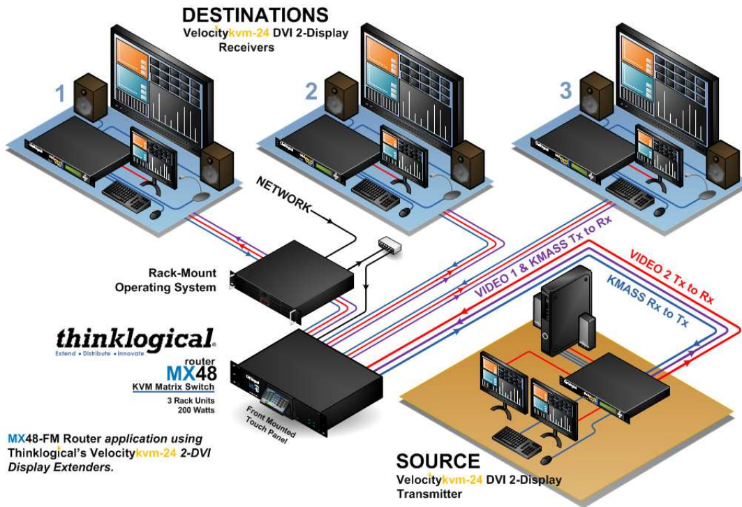
Figure 2a. Thinklogical MX 48 Router (Front Mount)
