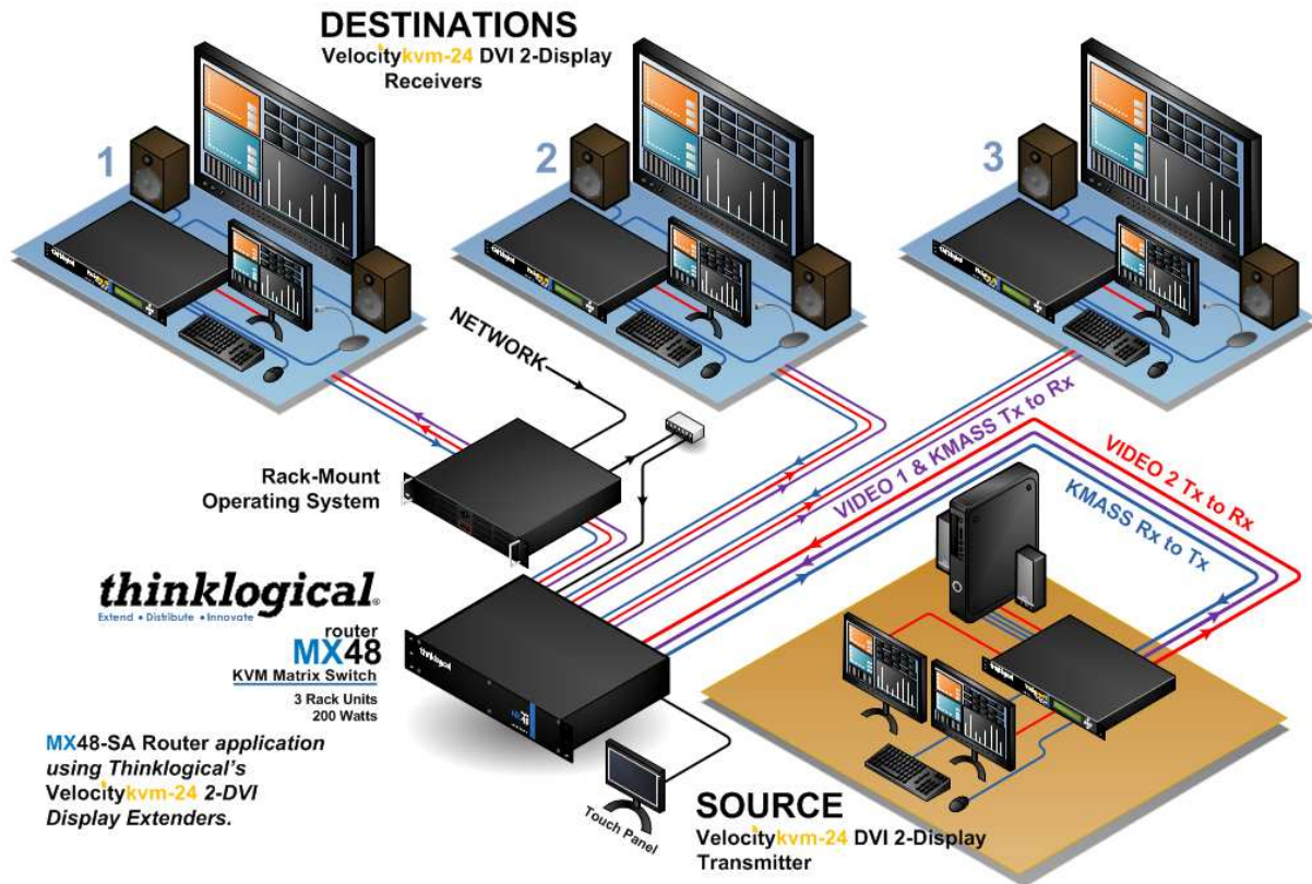
Figure 2c. Typical TOE MX 48 Router (Stand Alone)
