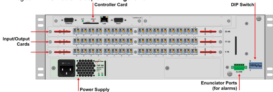
Figure 1a. Thinklogical MX 48 Router
