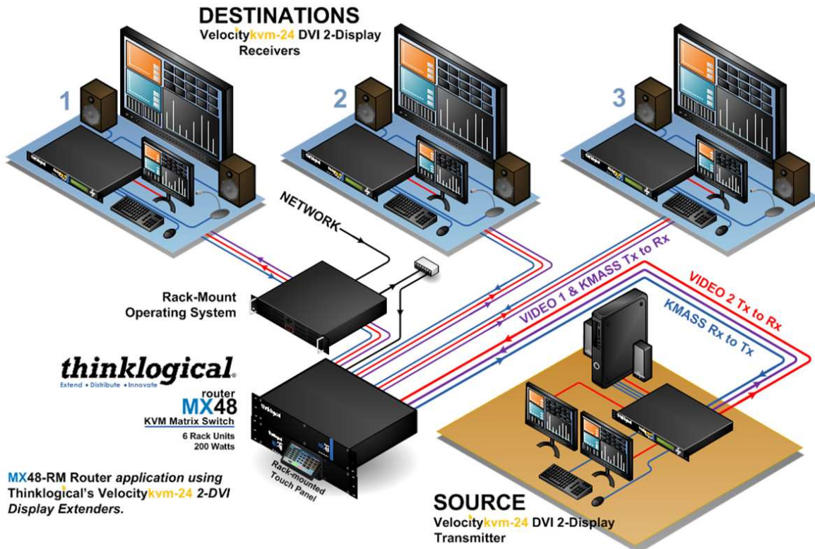
Figure 2b. Thinklogical MX 48 Router (Rack Mount)
