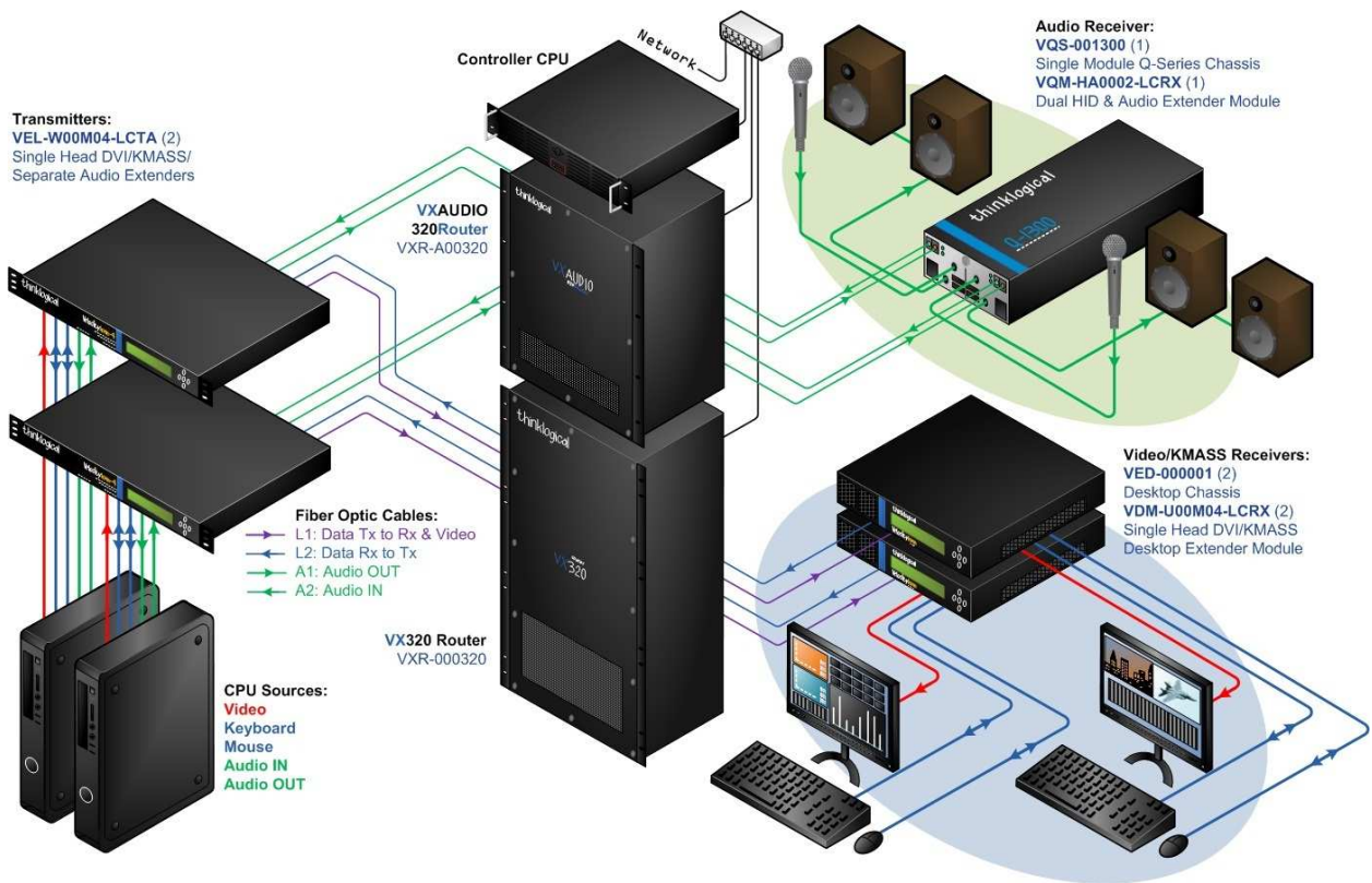
2a. Typical TOE VX320 Audio Configuration
