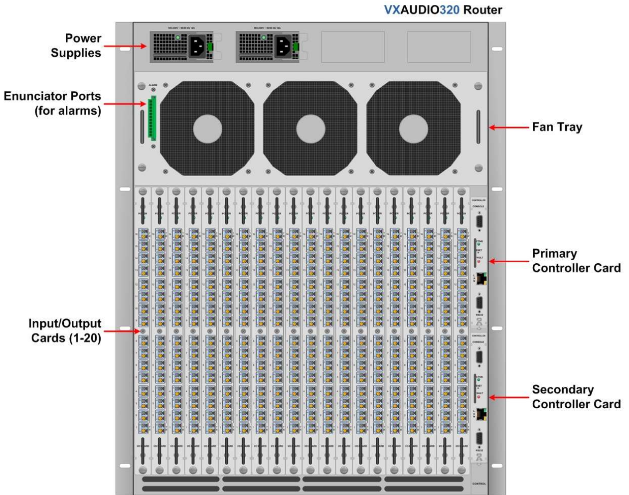
Figure 1a. Thinklogical VX 320 Audio Router
